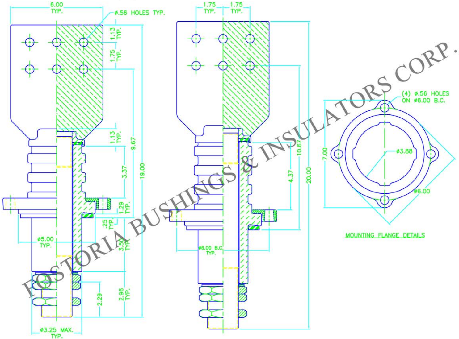
2.5 kV CLASS, 60 kV B.I.L. 4.00" - LEAKAGE DISTANCE
